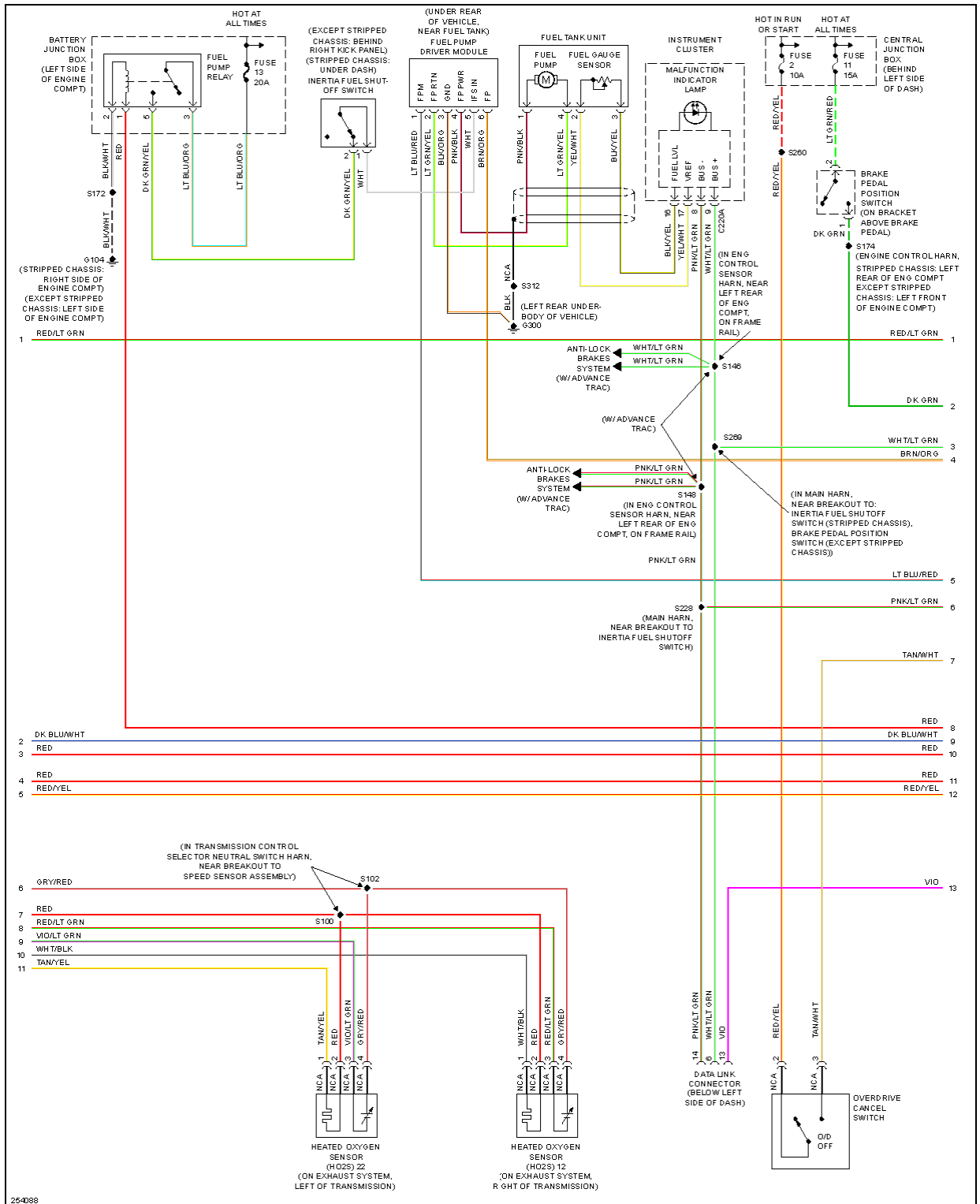
Fig. 33: 6.8L, Engine Performance Circuit (4 of 5)
