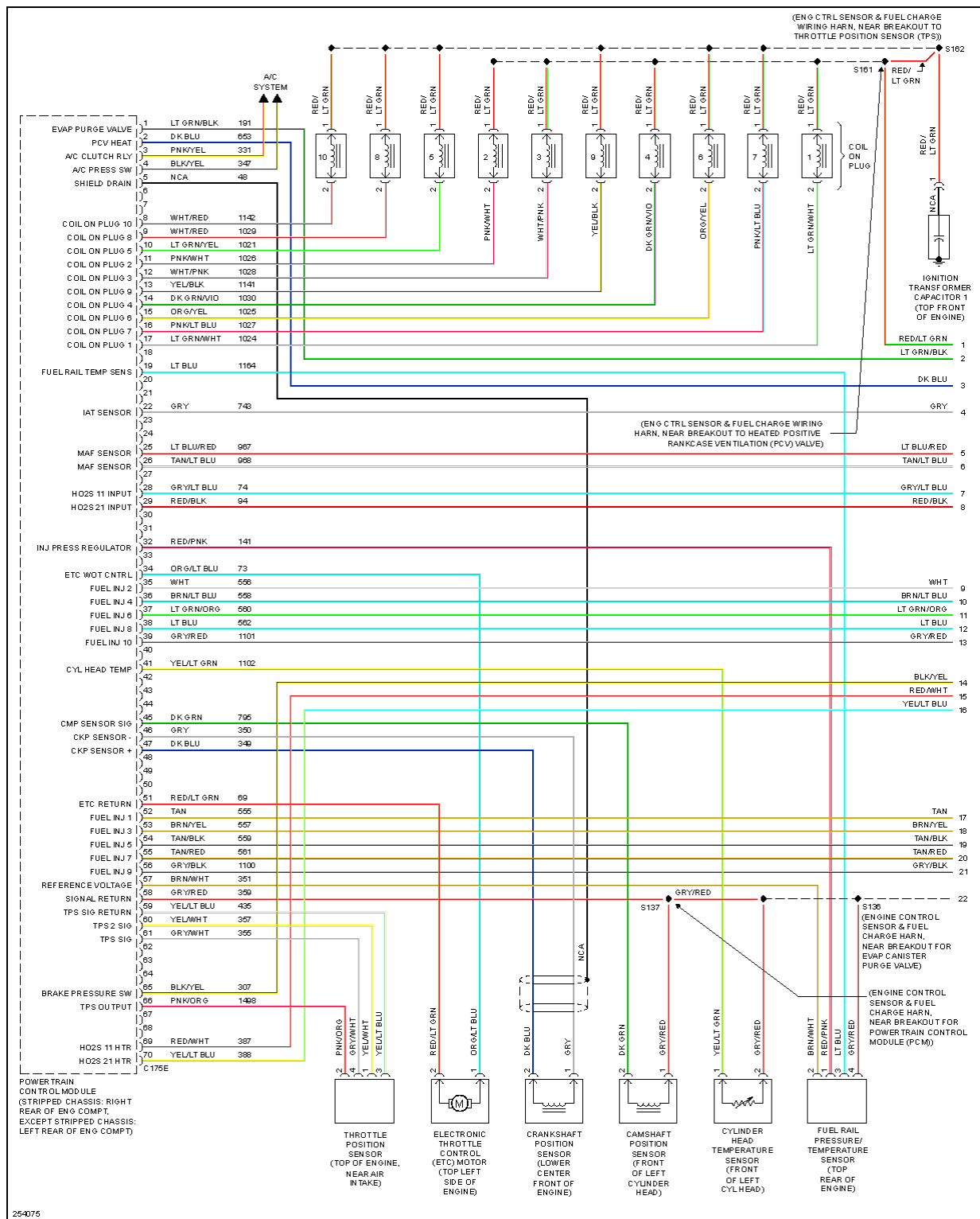
Fig. 30: 6.8L, Engine Performance Circuit (1 of 5)
