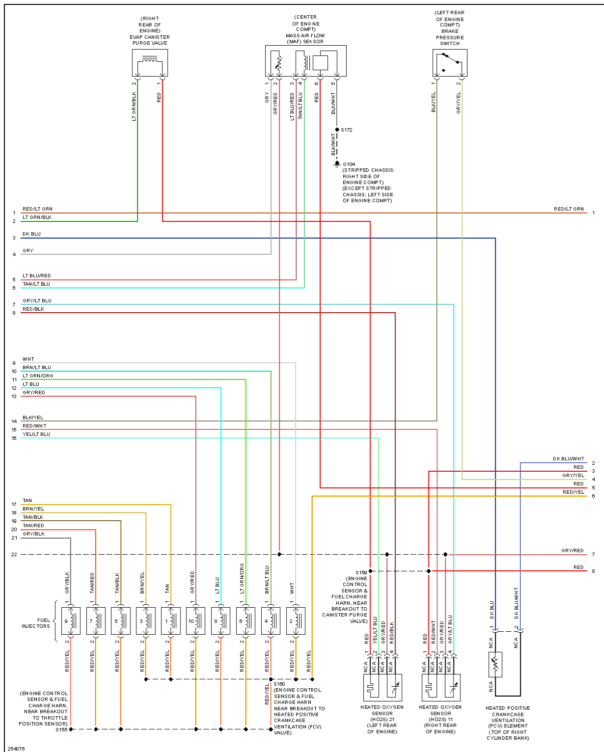
Fig. 31: 6.8L, Engine Performance Circuit (2 of 5)
