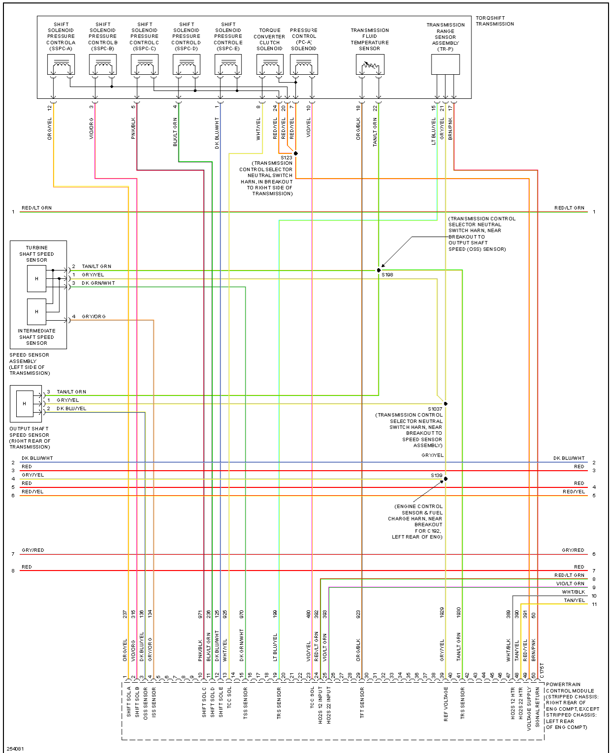
Fig. 32: 6.8L, Engine Performance Circuit (3 of 5)
