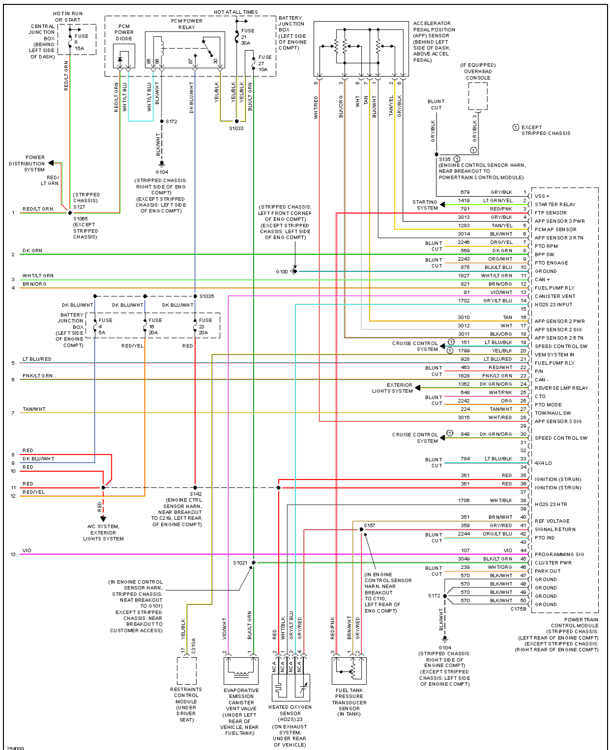
Fig. 34: 6.8L, Engine Performance Circuit (5 of 5)
