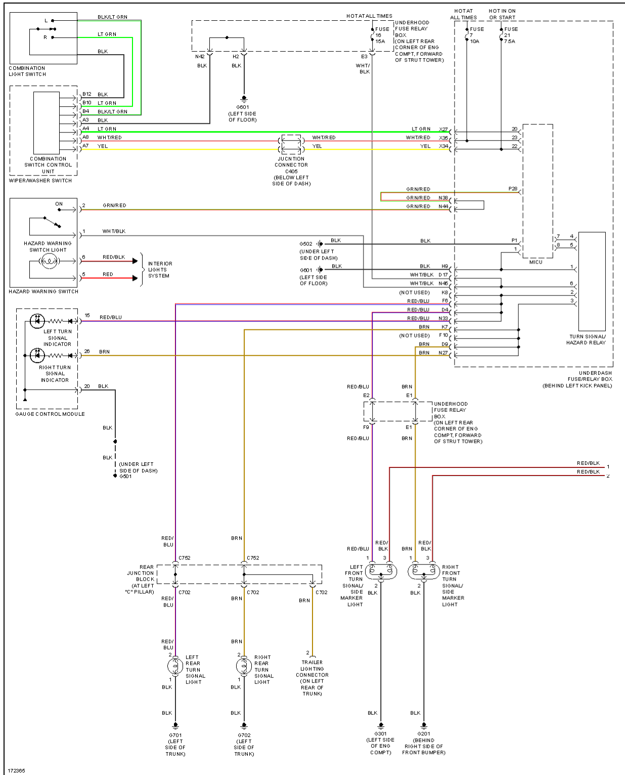
Fig. 35: Exterior Lamps Circuit, Coupe (1 of 2)
