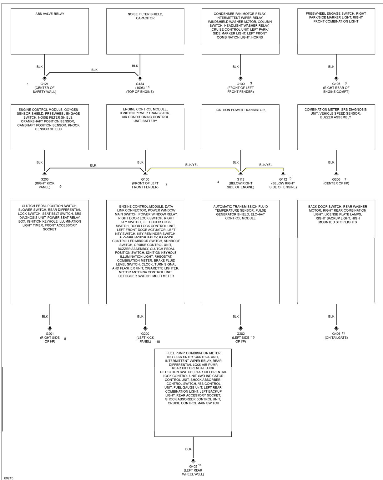
Fig. 25: Ground Distribution Circuit
