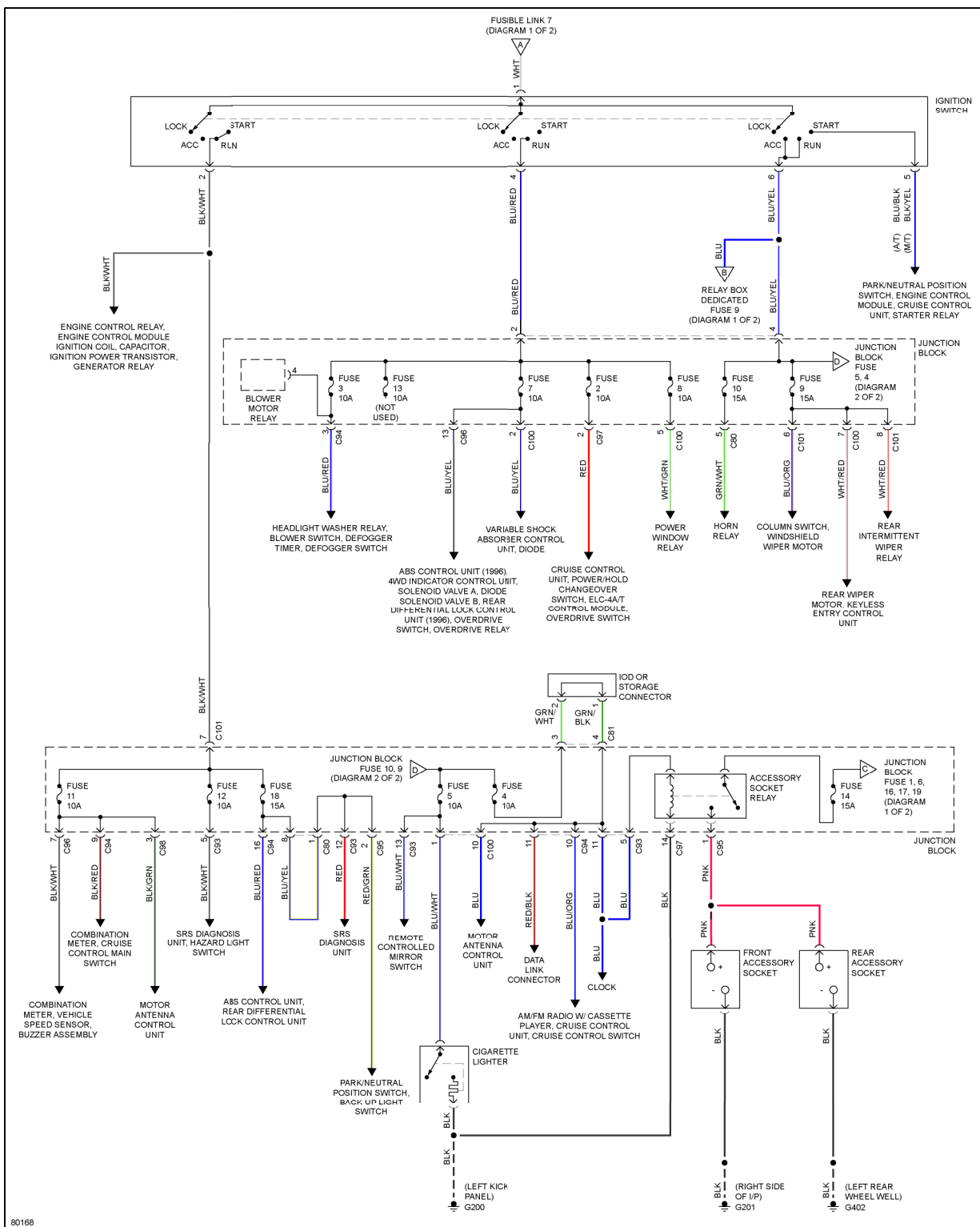
Fig. 35: Power Distribution Circuit (2 of 2)
