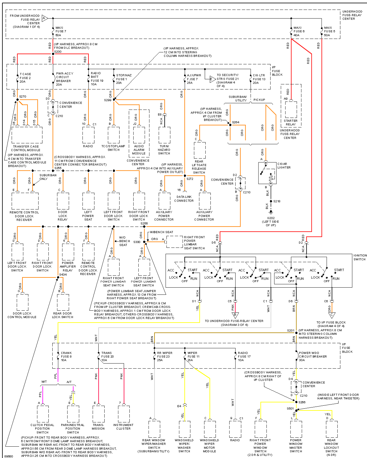
Fig. 57: Power Distribution Circuit (2 of 4)
