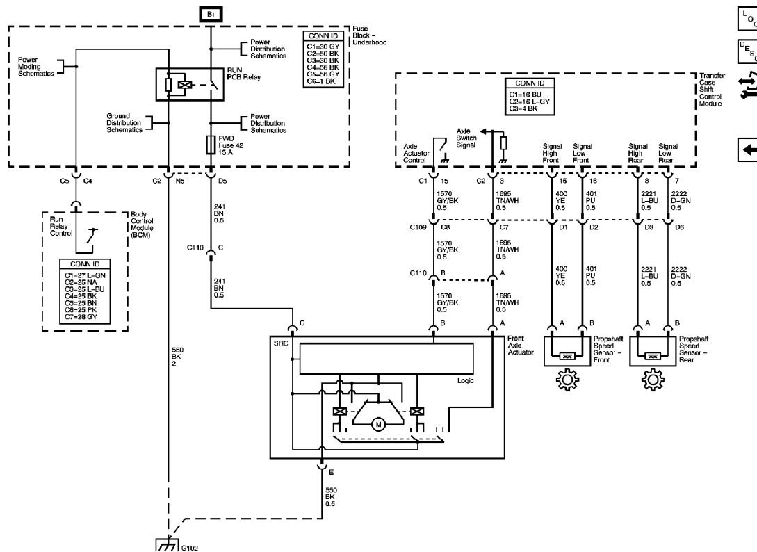
Fig. 4: Front Axle Actuator & Speed Sensors Schematic Courtesy of GENERAL MOTORS CORP.
