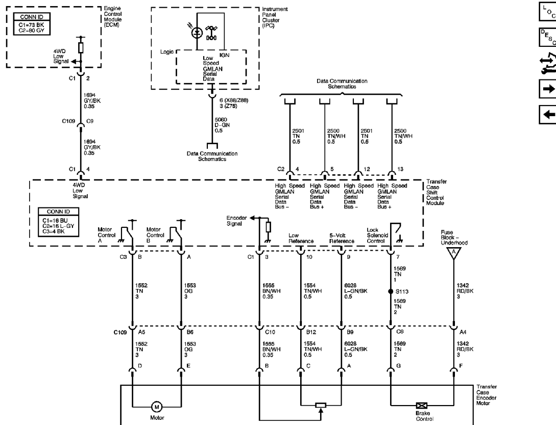
Fig. 3: Encoder Motor Control & Serial Data Schematic Courtesy of GENERAL MOTORS CORP.
