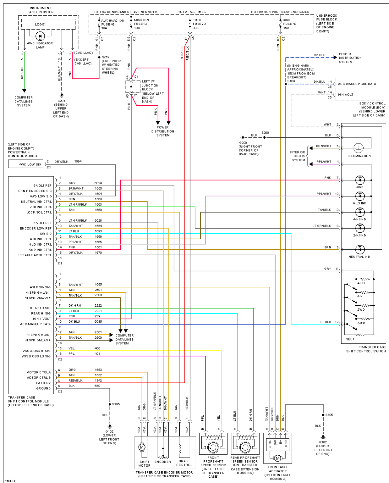
SYSTEM WIRING DIAGRAMS Fig. 129: Transfer Case Circuit
