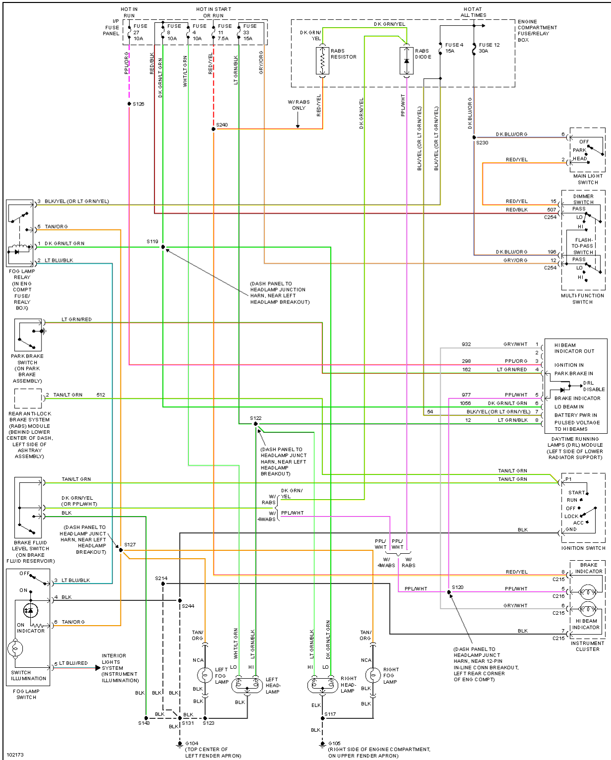
Fig. 27: Headlamps/Fog Lamps Circuit, W/ DRL
