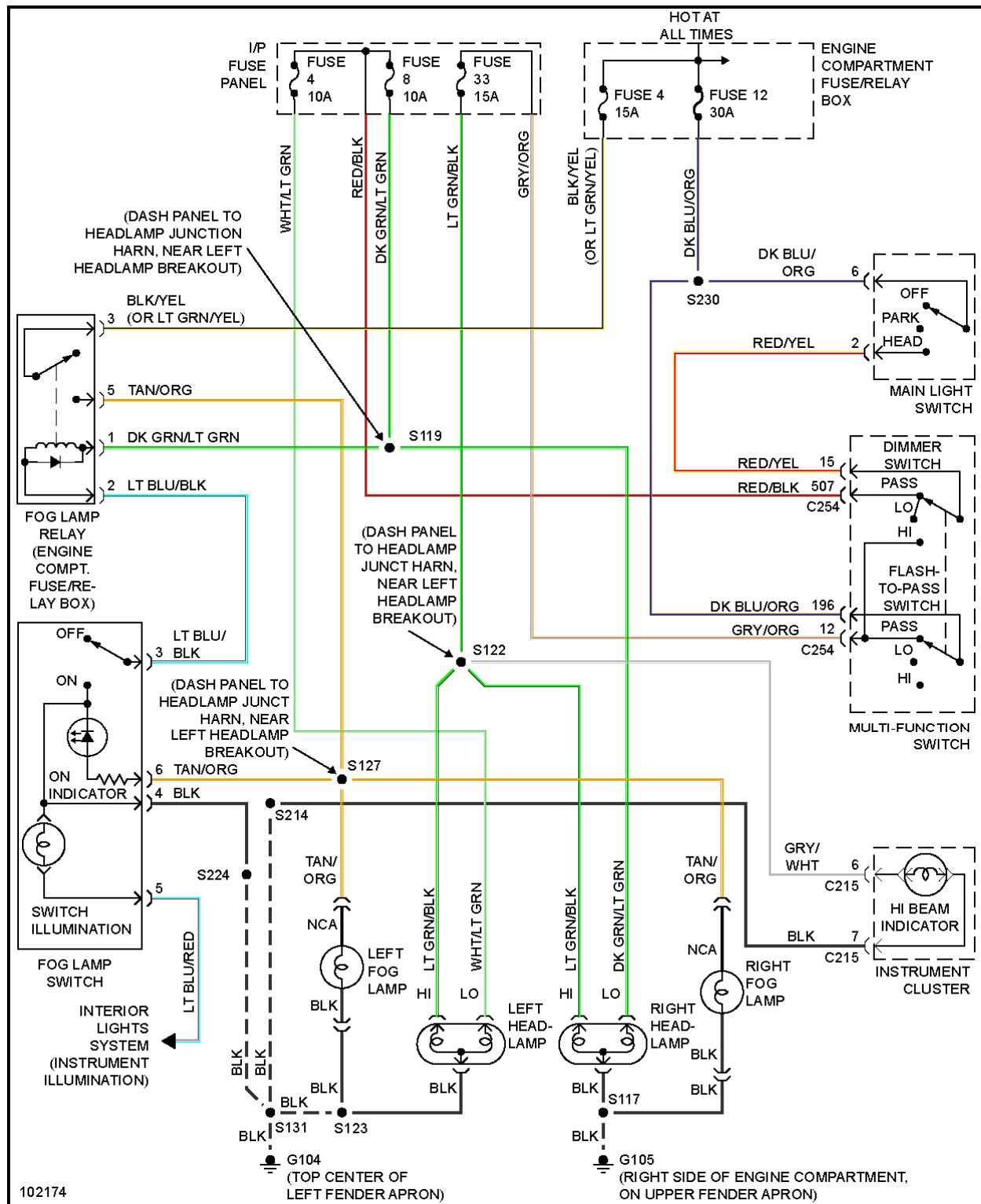
Fig. 28: Headlamps/Fog Lamps Circuit, W/O DRL
